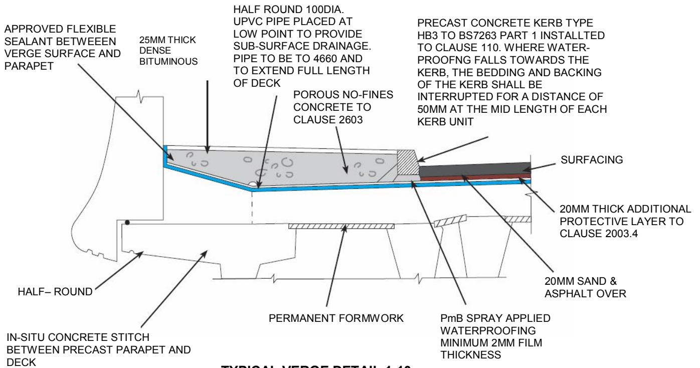
TYPICAL VERGE DETAIL 1:10
